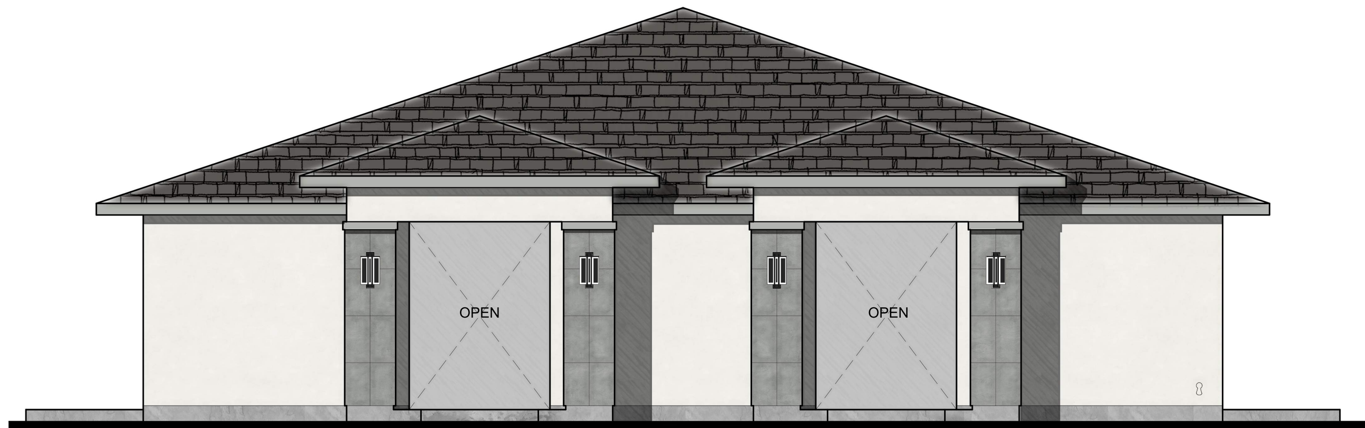
SOUTH ELEVATION 1/4" = 1'-0"
