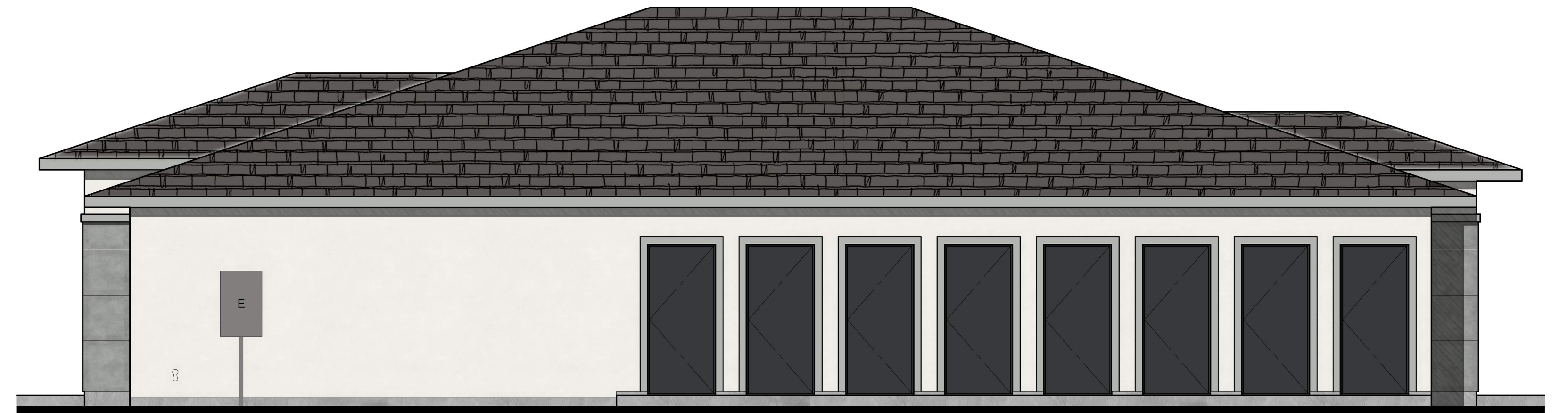
WEST ELEVATION 1/4" = 1'-0"
