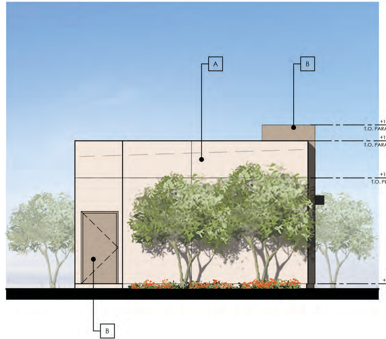
GARAGE BUILDING TYPE 3 LEFT ELEVATION
