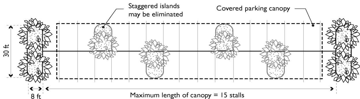
Figure 18.90.050.B.7. Covered Canopies
