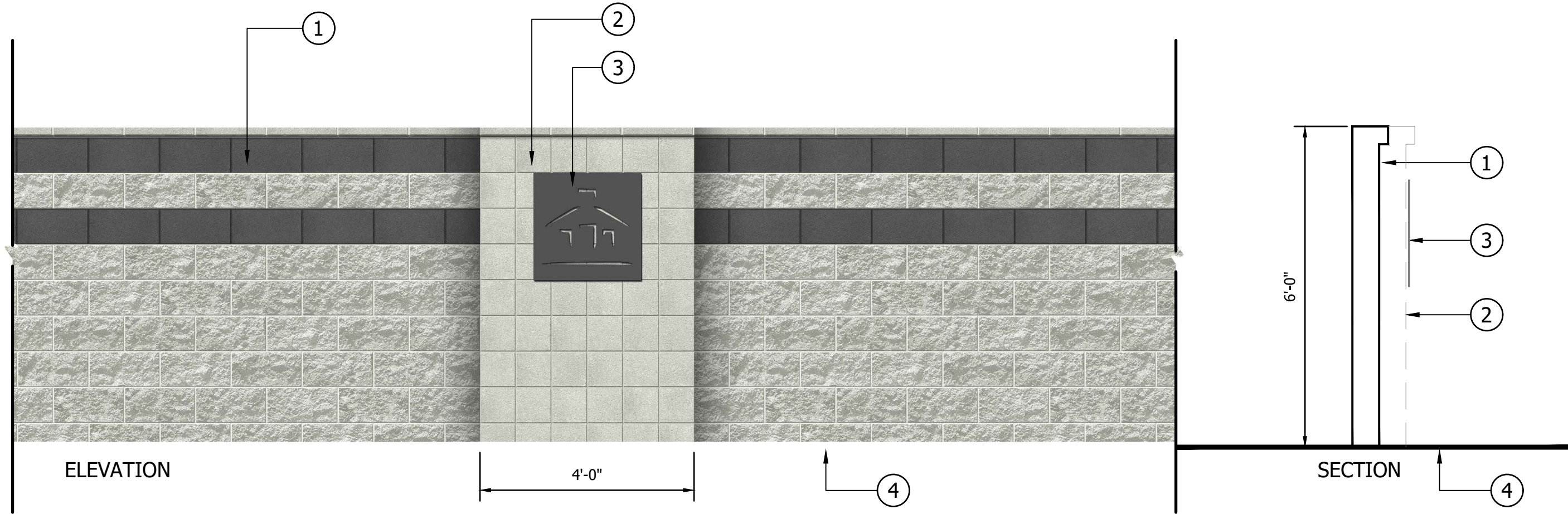
2 BRANDING AT PARCEL ENTRY 1/2" = 1'-0"
