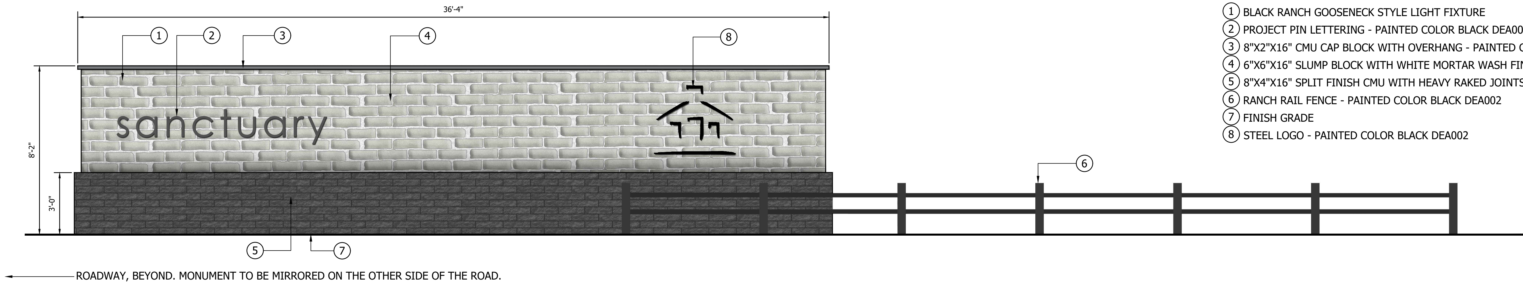
1 ENTRY MONUMENT 3/8" = 1'-0"
