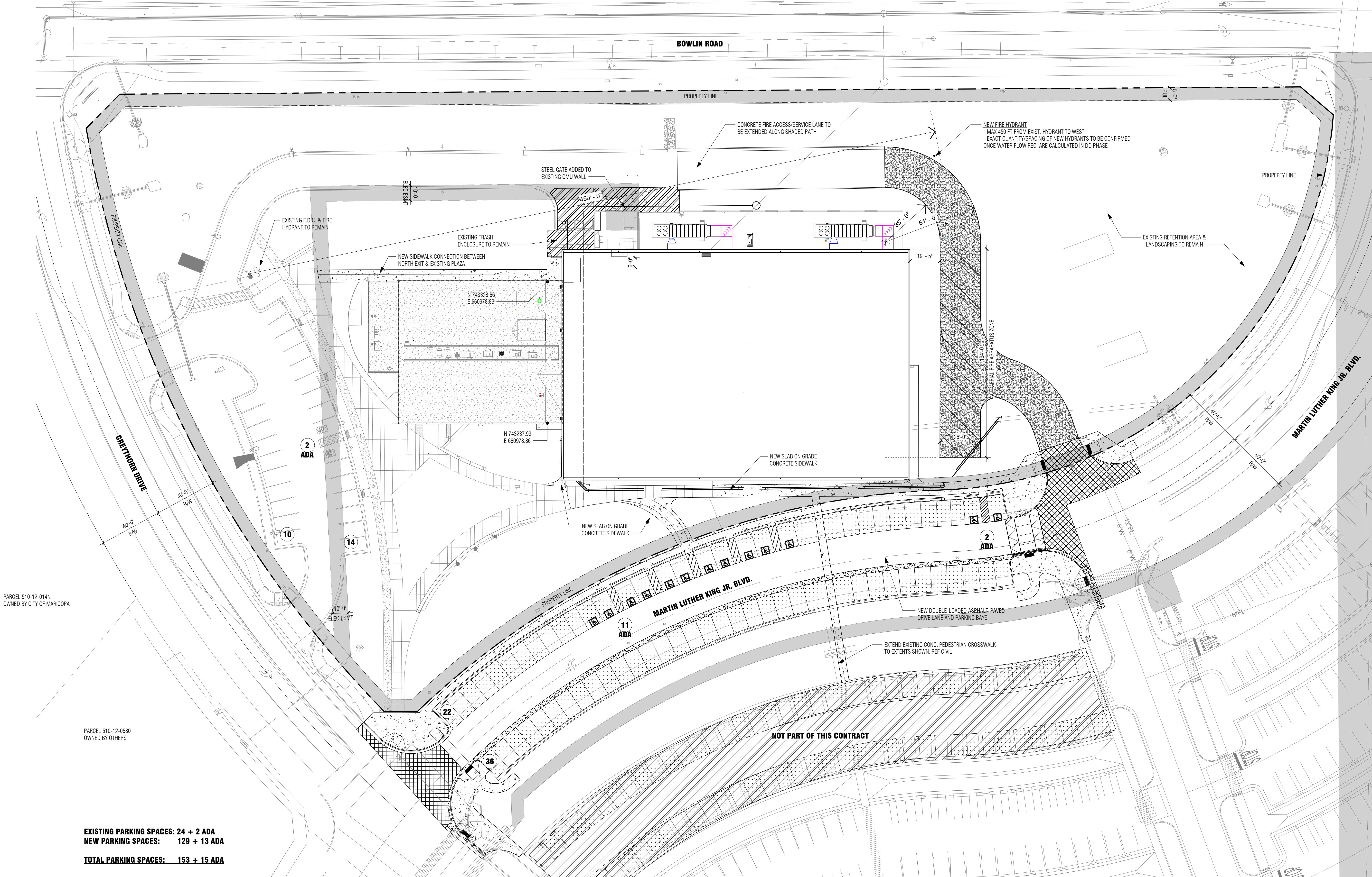
1 ARCHITECTURAL SITE PLAN 1" = 30'-0"
