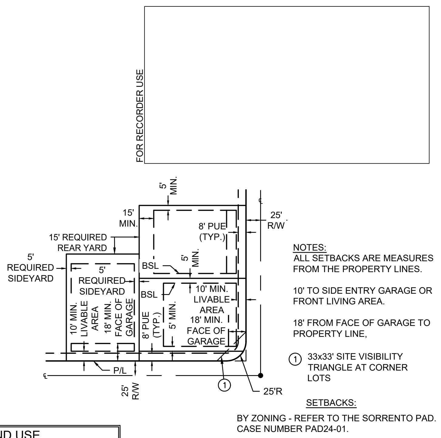
TYPICAL LOT LAYOUT AND BUILDING SETBACKS N.T.S.
