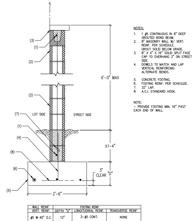
2 FREE-STANDING MASONRY WALL AND FOOTING NO SCALE
