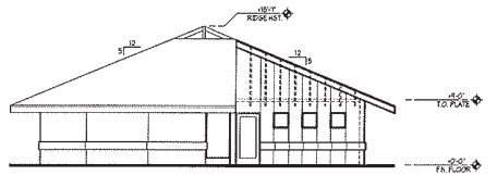
3 RIGHT FRONT REF: 1A-3 FOR SH. NOTES PATIO TRILLS SHOWN DIMED FOR CLARITY
