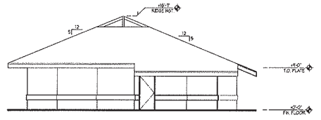
2 RIGHT REAR REF: 1A-3 FOR SH. NOTES
