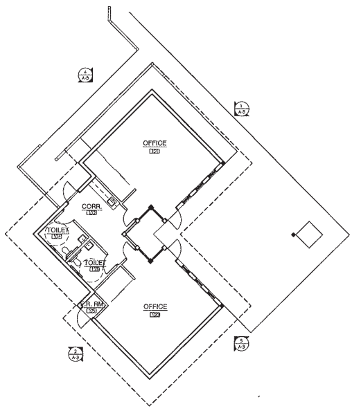
1 FLOOR PLAN 1/8" = 1'-0"
