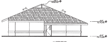
4 LEFT REAR REF: 1A-3 FOR SH. NOTES
