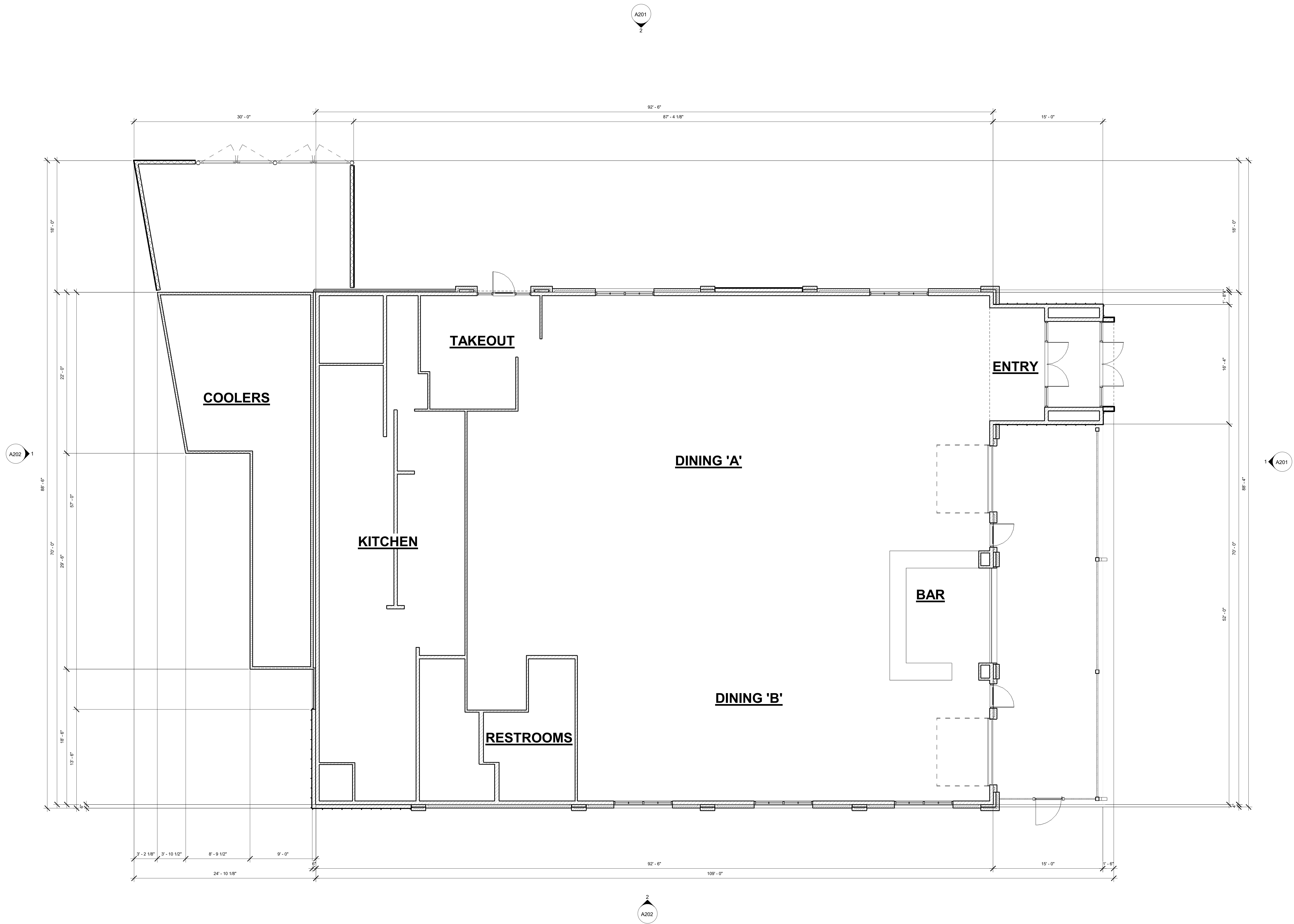
1 FLOOR PLAN A101 SCALE 3/16" = 1'-0"
