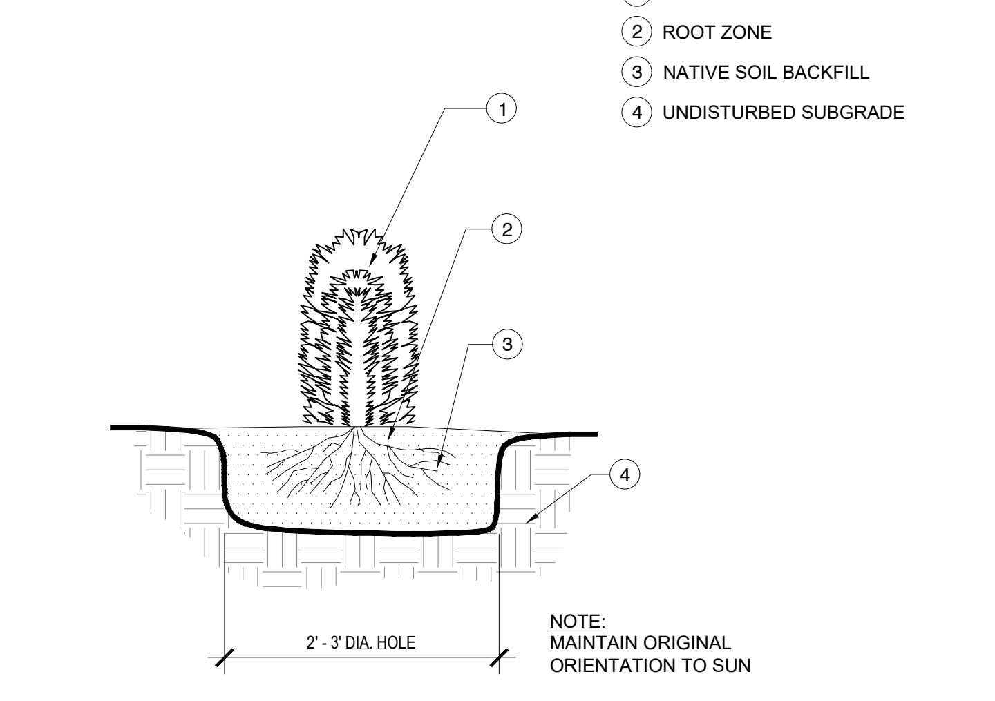
6 CACTUS PLANTING NTS P-RE-DP-01
