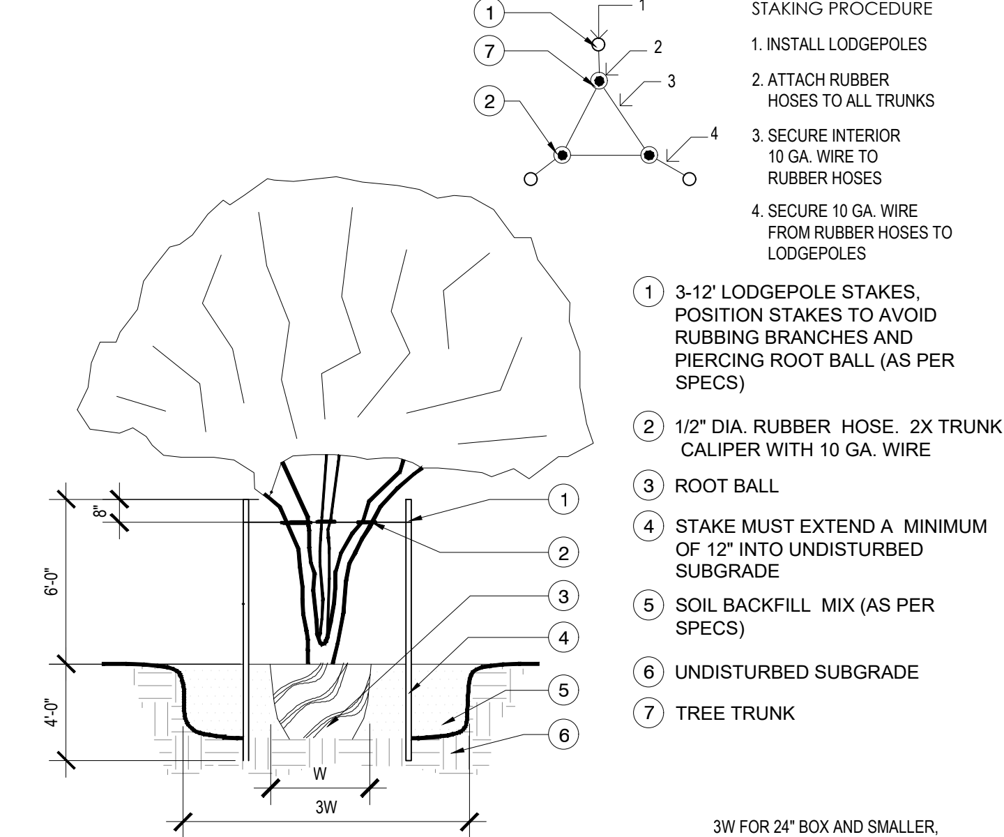
3 MULTI-TRUNK TREE PLANTING NTS P-RE-DP-10
