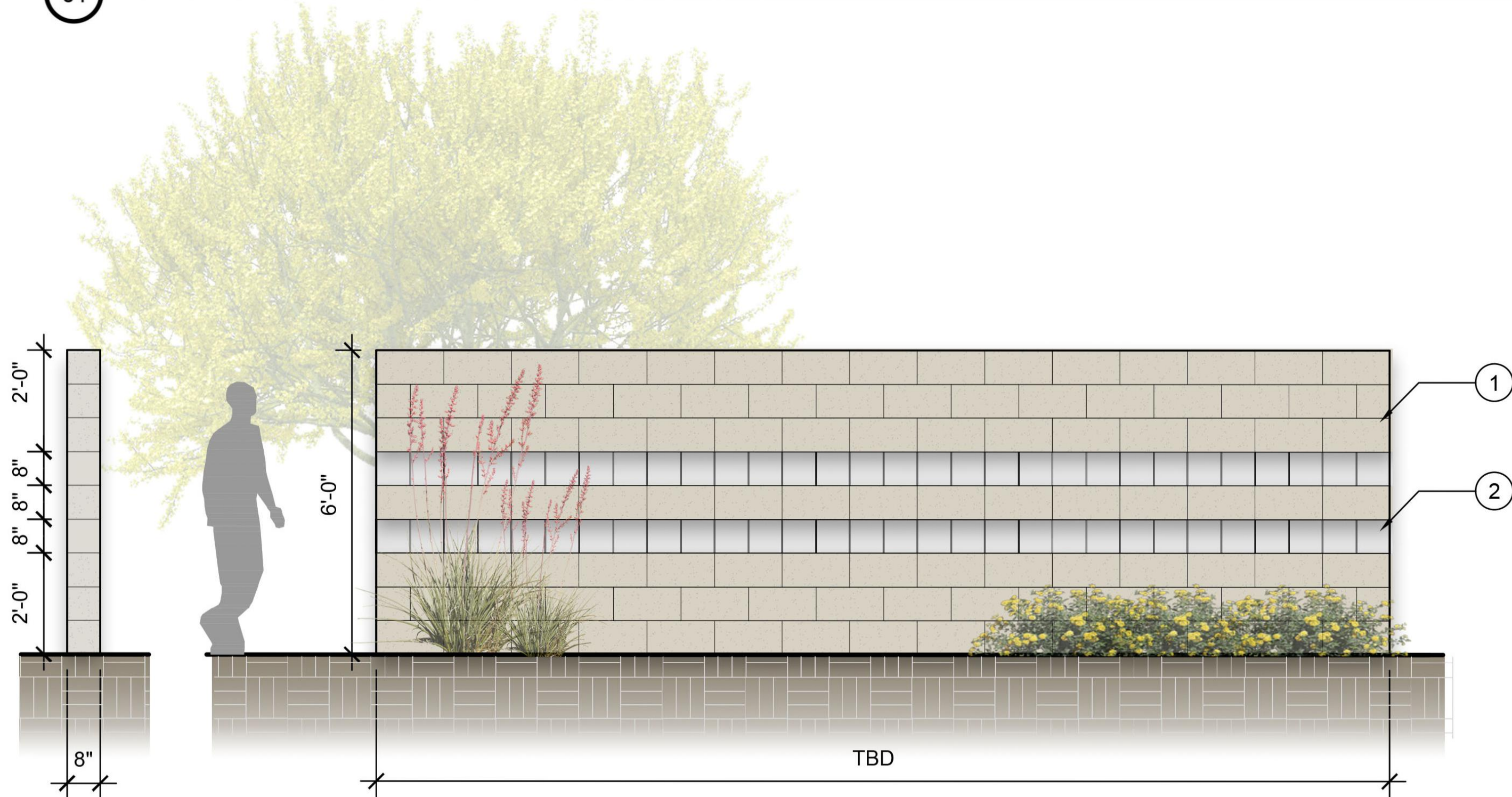
02 PERIMETRAL WALL (REQUESTED MODIFICATIONS).
