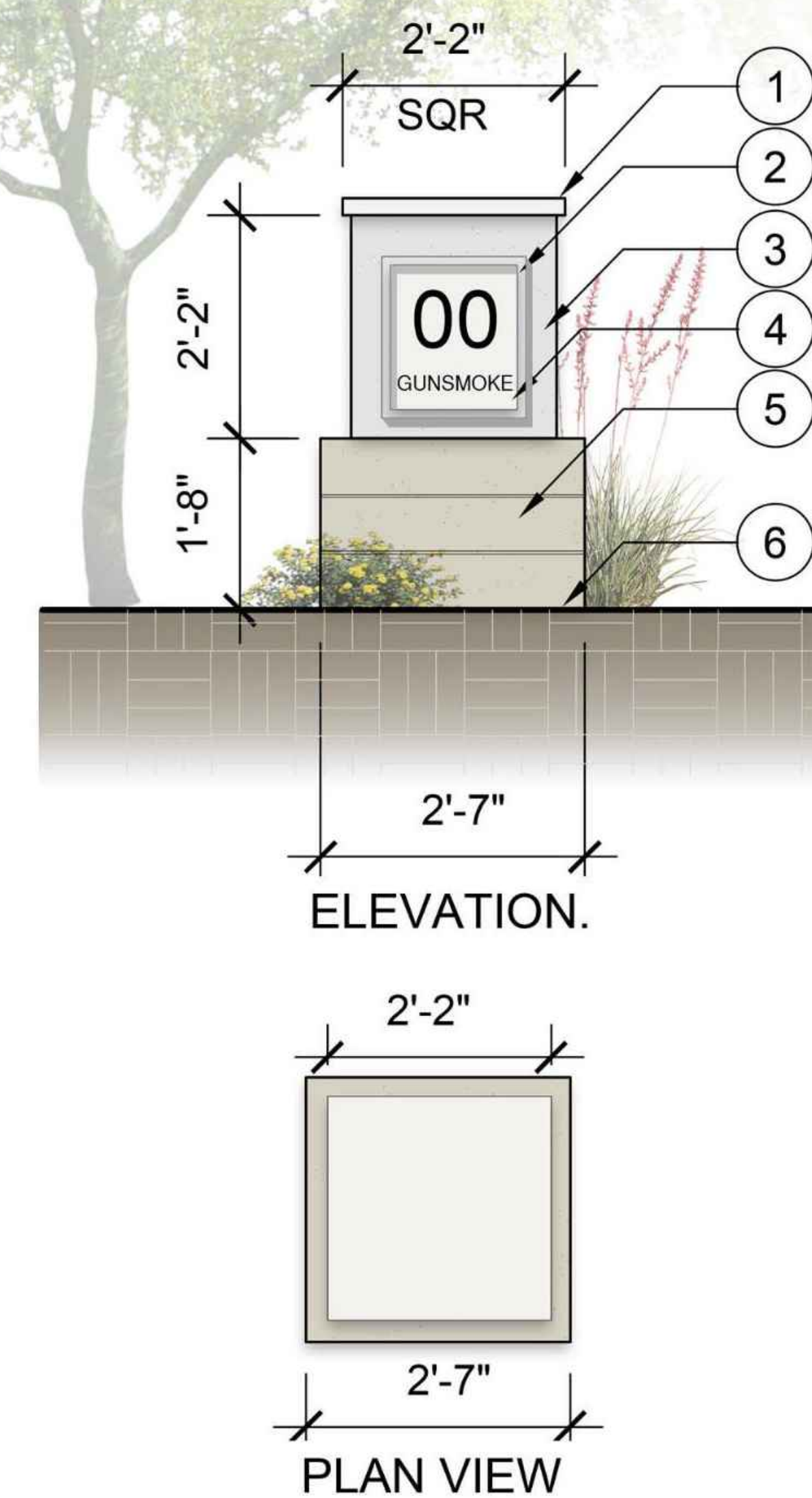
02 STREET MAP MONUMENT
