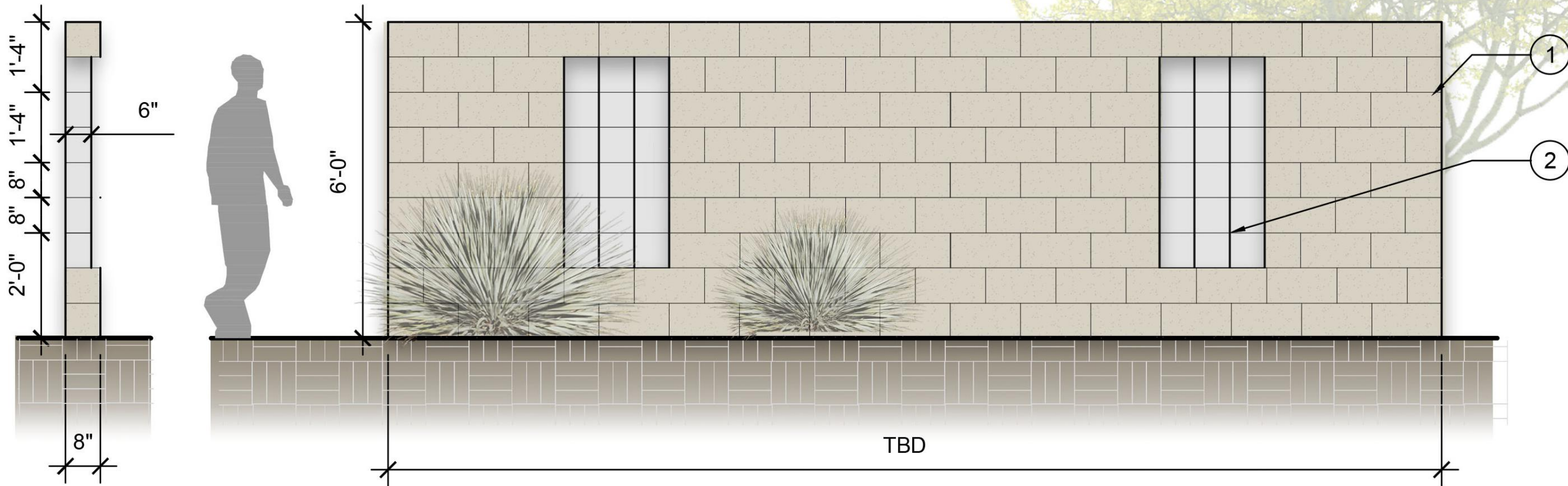
02 PERIMETRAL WALL (ALTERNATIVE 2)
