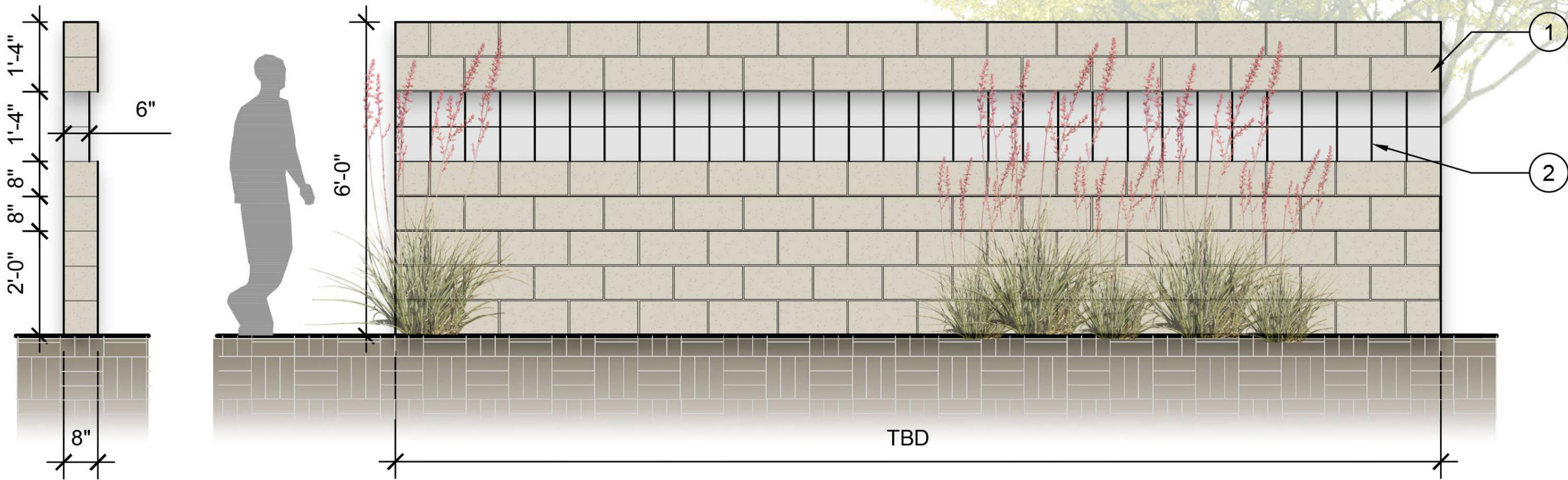
01 PERIMETER WALL (ALTERNATIVE 1)
