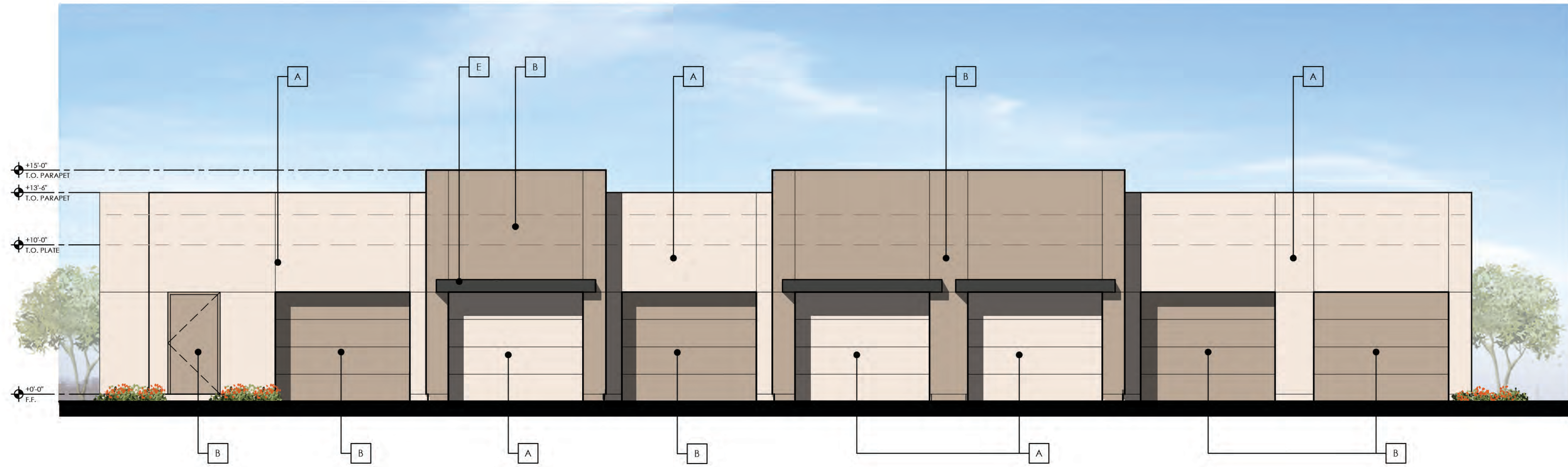
GARAGE BUILDING TYPE 3 TYPICAL SITE INTERIOR ELEVATION
