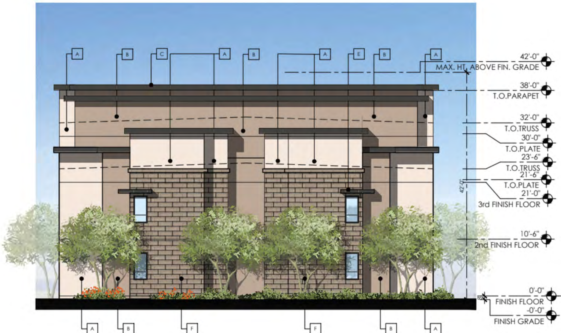
BUILDING TYPE 1C LEFT ELEVATION
