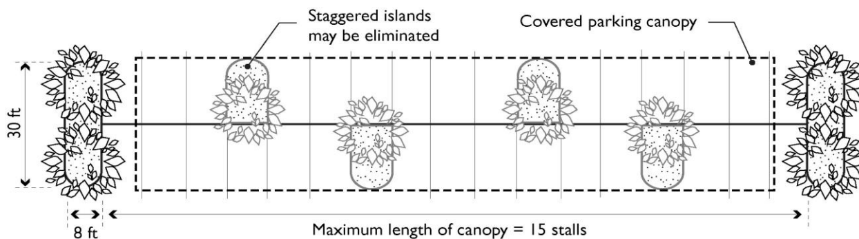
Figure 18.90.050.B.7. Covered Canopies
