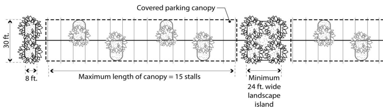
Figure 18.90.050.B.6. Adjacent Canopies
