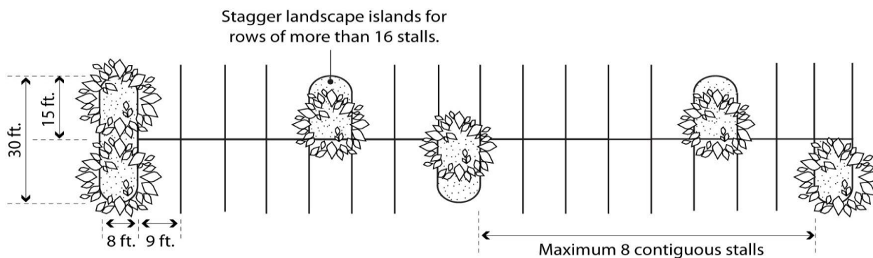
Figure 18.90.050.B.4. Landscape Islands
