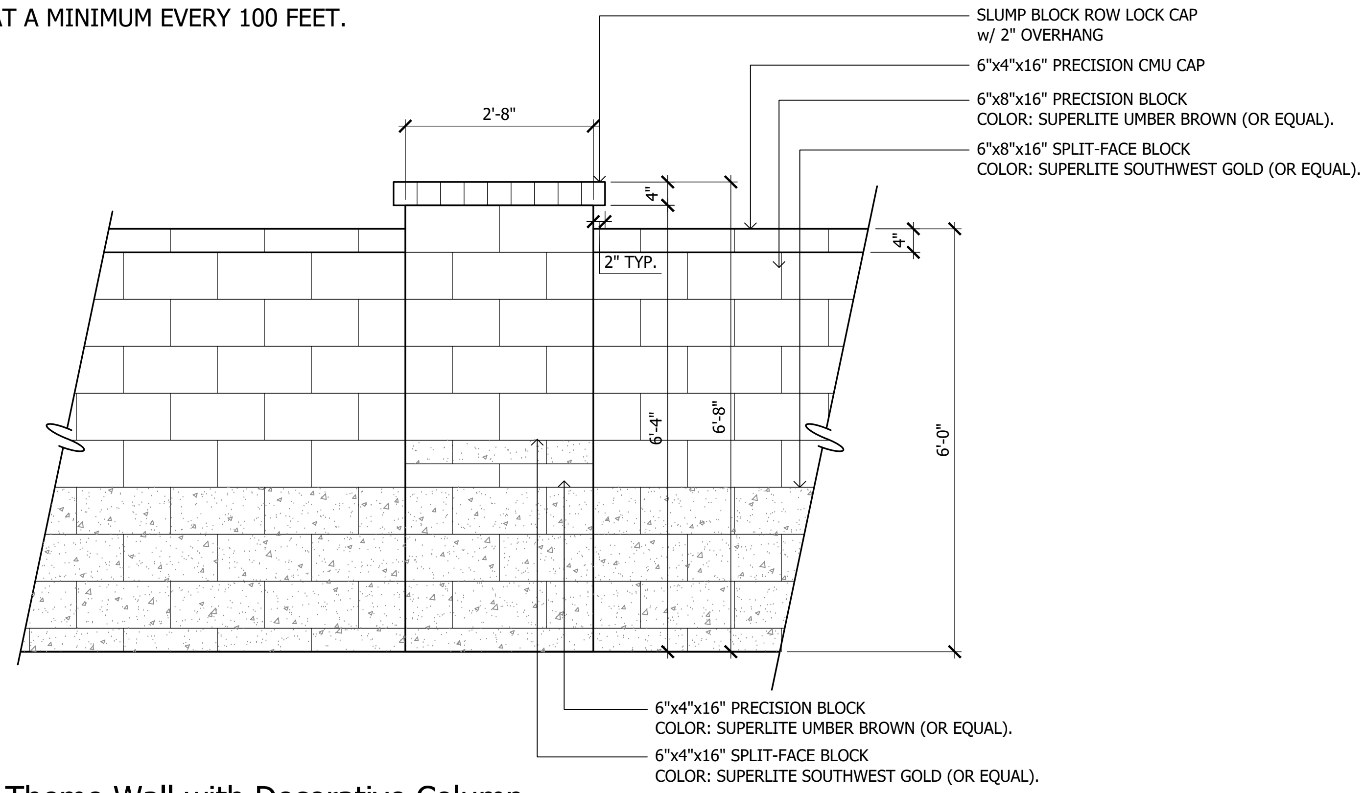
1 Theme Wall with Decorative Column SCALE: 1/2"=1'-0"
