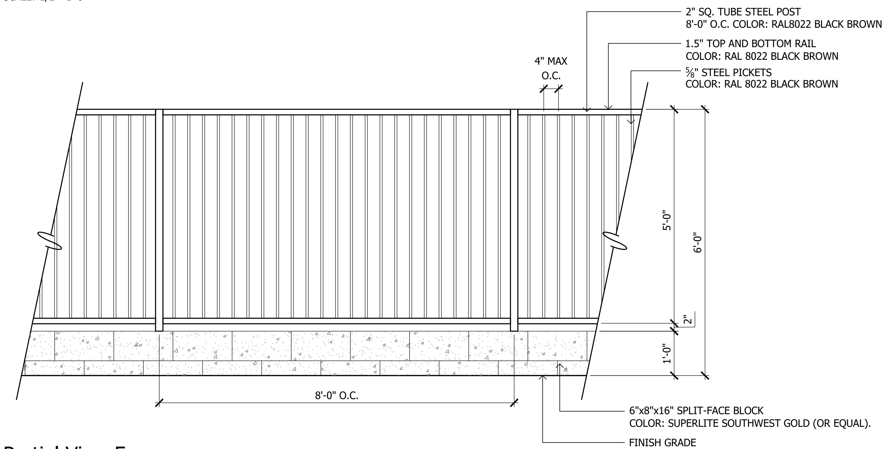
3 Partial View Fence SCALE: 1/2"=1'-0"
