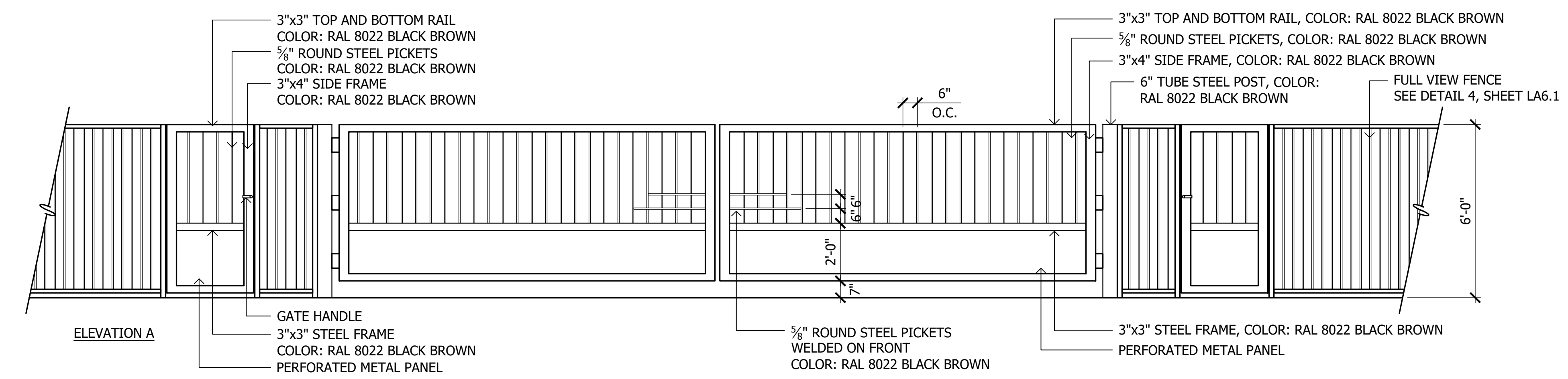
1 Emergency Access Gate Elevation SCALE: 3/8"=1'-0"
