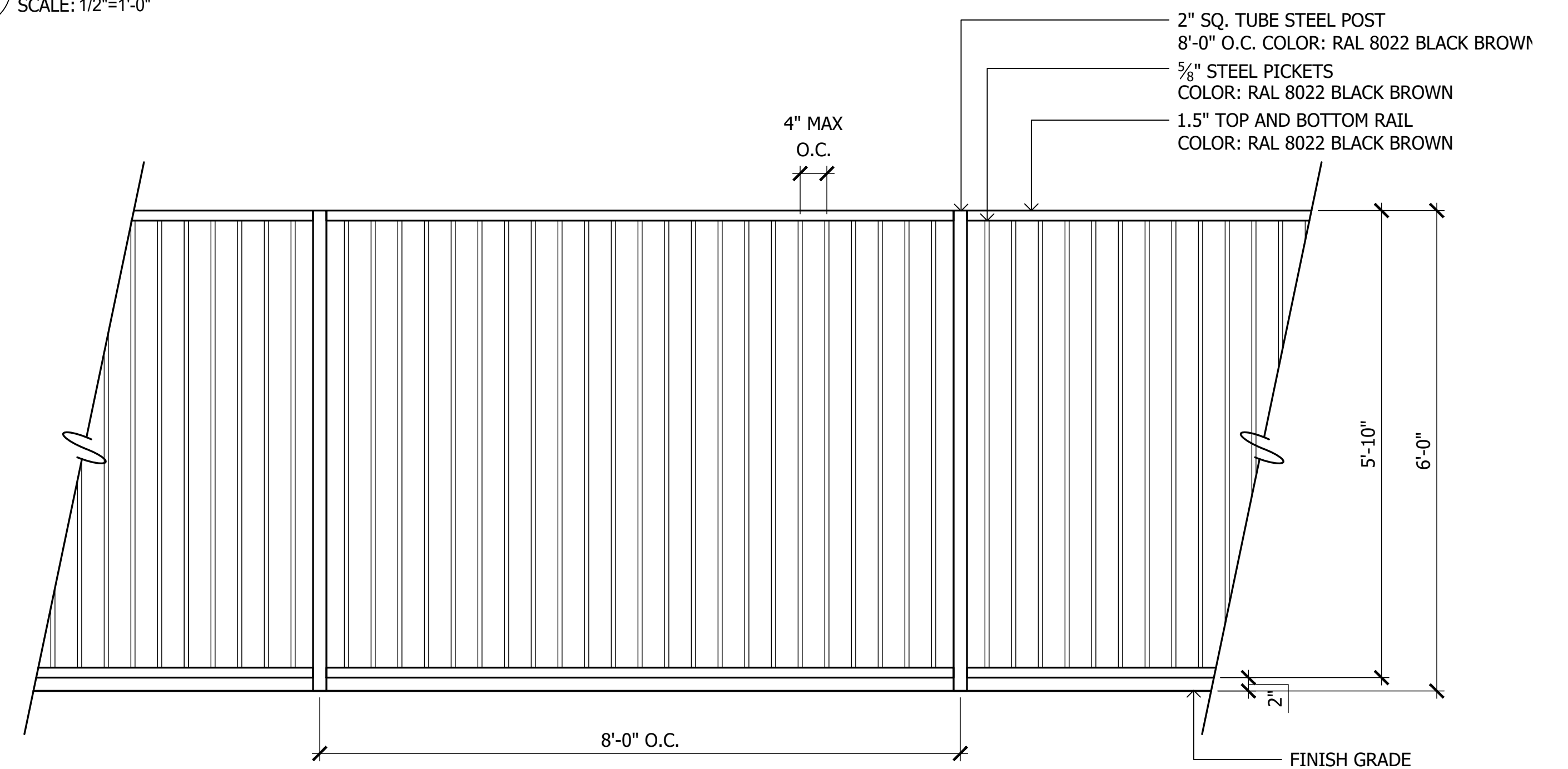
2 Secondary Wall SCALE: 1/2"=1'-0"
