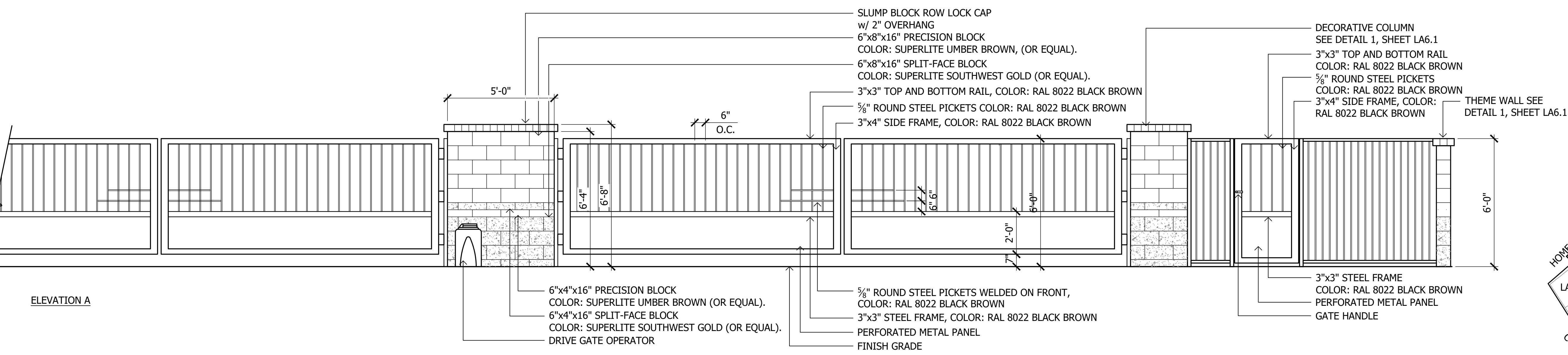
1 Vehicle Gate Elevation SCALE: 3/8"=1'-0"
