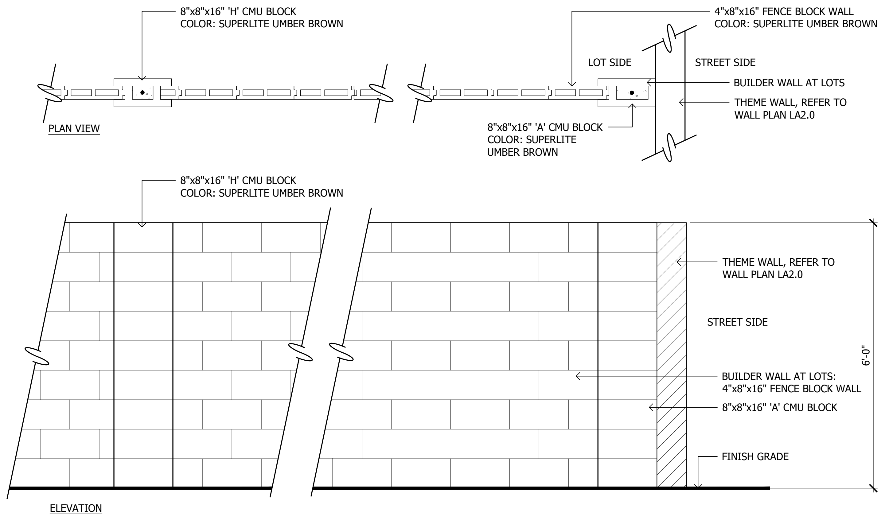
2 Secondary Wall SCALE: 1/2"=1'-0"
