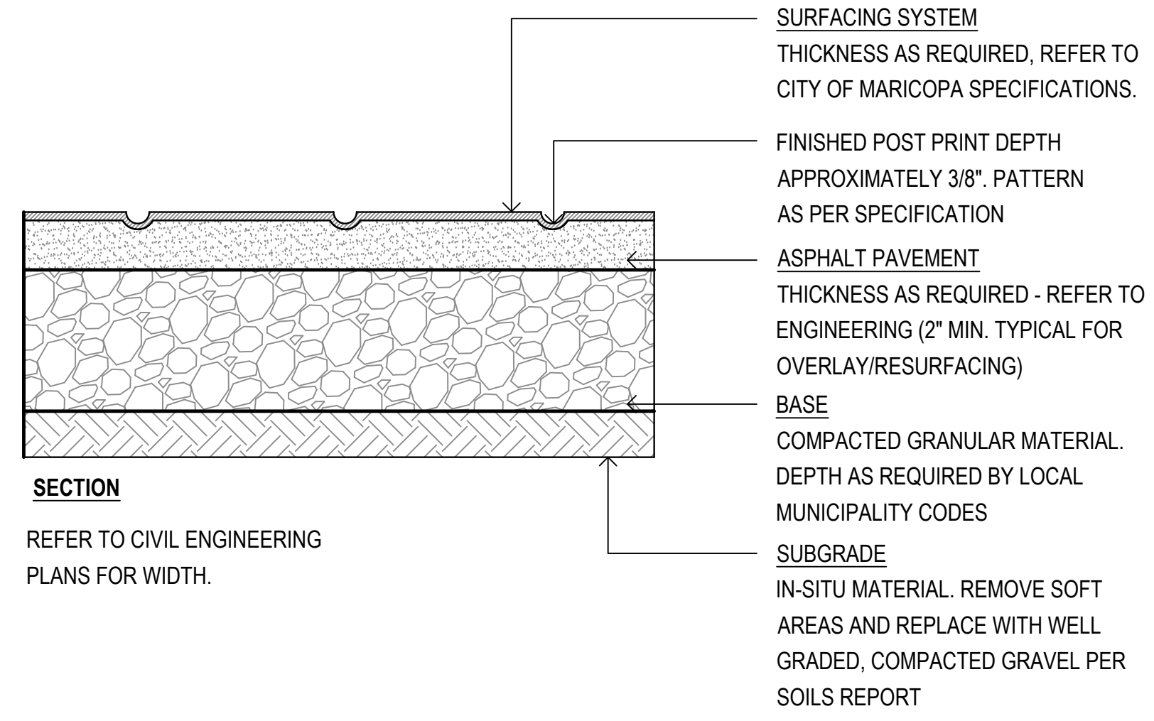
3 Stamped Asphalt SCALE: 1/2"=1'-0"
